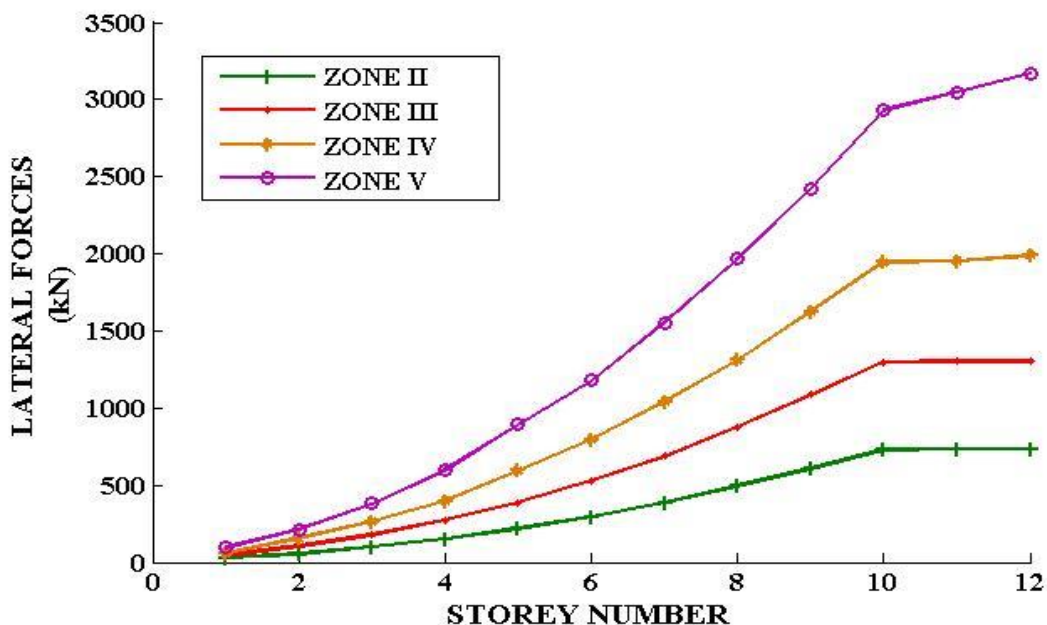
Fig: 6 Lateral forces on shear wall due to seismic forces
