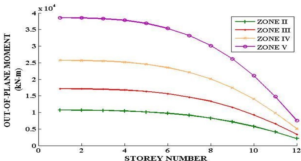
Fig: 2 Out-of-plane moment on shear wall due to seismic forces
