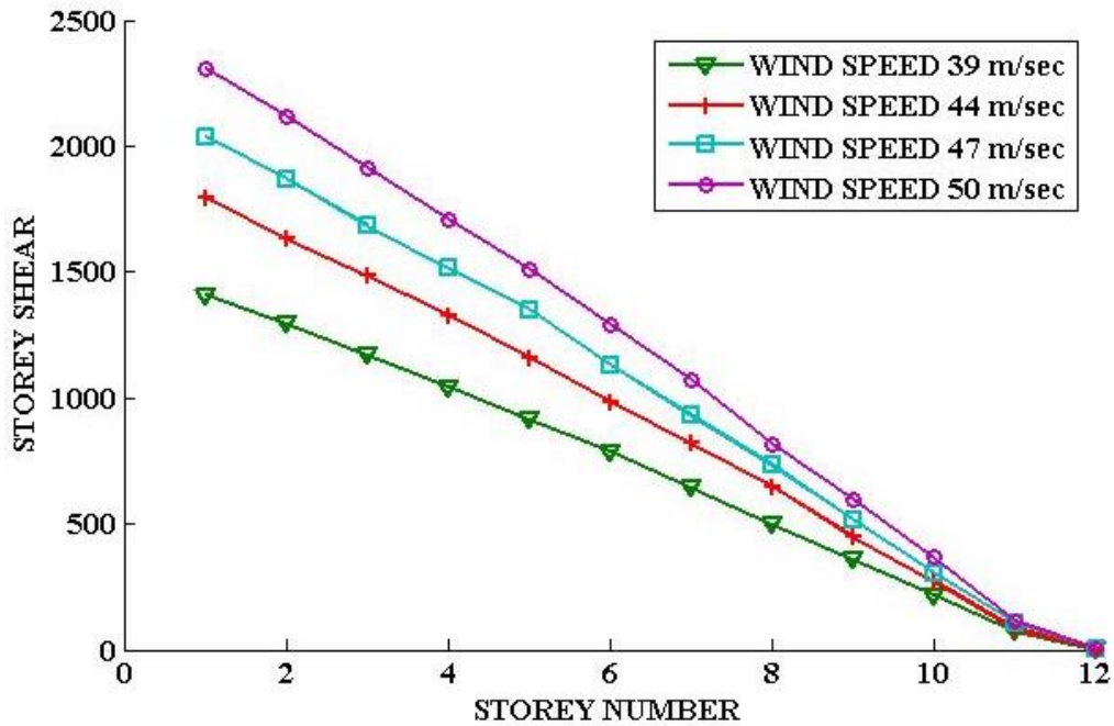
Fig: 13 Storey shear on shear wall due to wind forces
