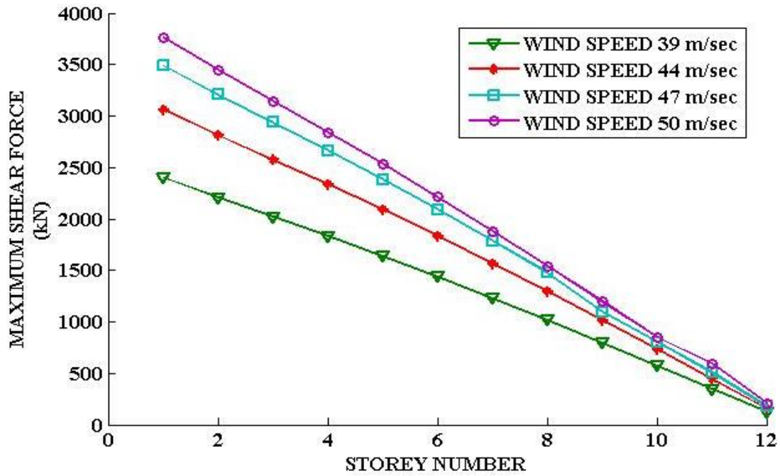
Fig: 9 Maximum shear forces on shear wall due to wind forces
