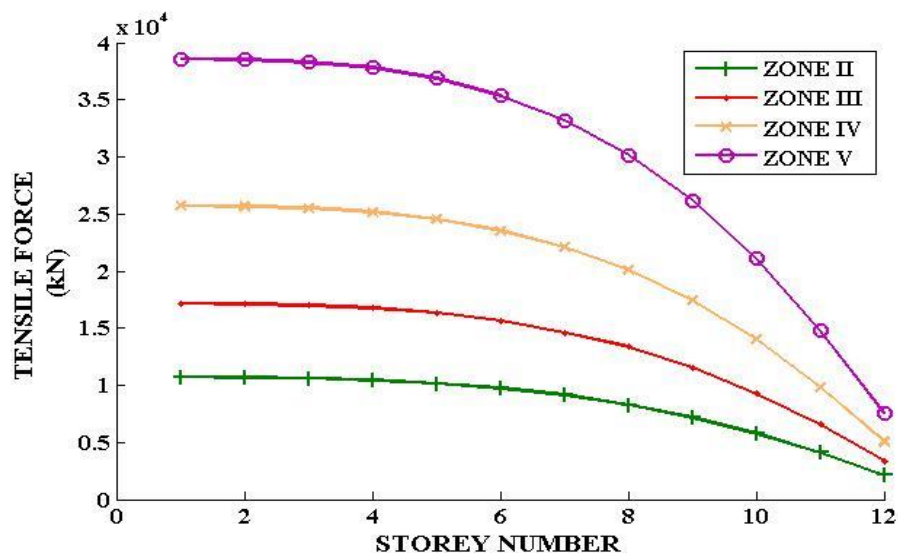
Fig: 4 Tensile force on shear wall due to seismic forces
