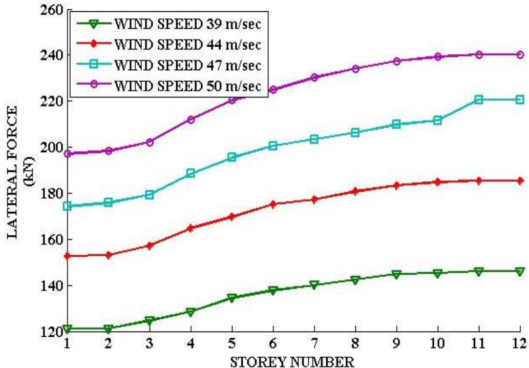
Fig: 12 Lateral forces on shear wall due to wind forces
