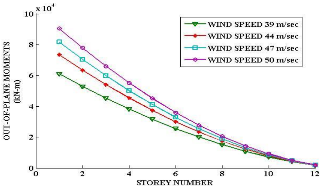
Fig: 8 Out-of-plane moments on shear walls due to wind forces
