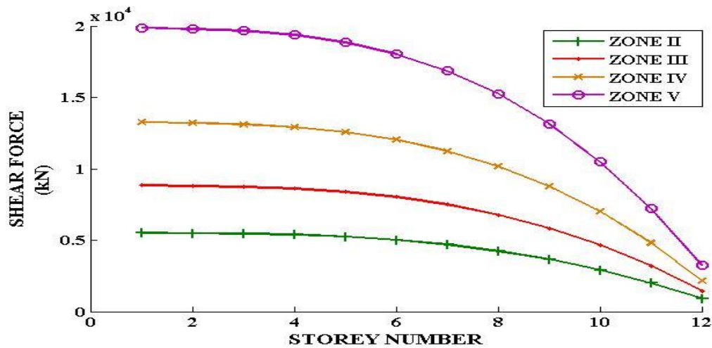
Fig: 3 Shear force on shear wall due to seismic forces
