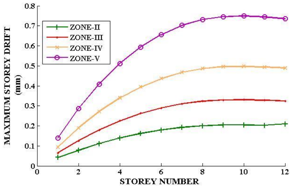
Fig: 5 Maximum storey drift on shear wall due to seismic forces
