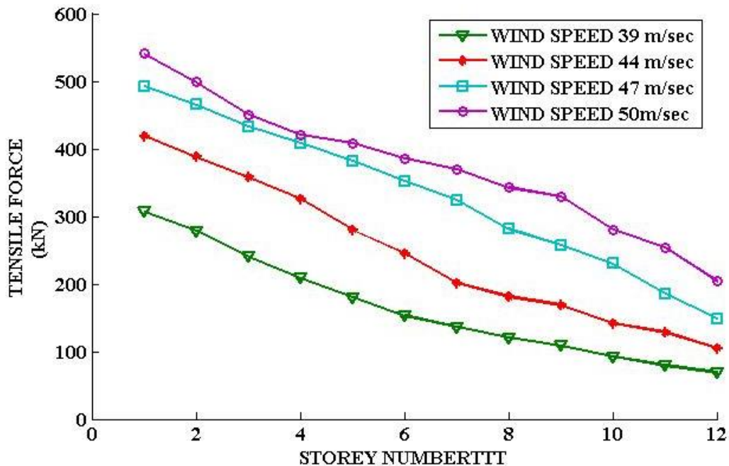
Fig: 10 Tensile forces on shear wall due to wind forces
