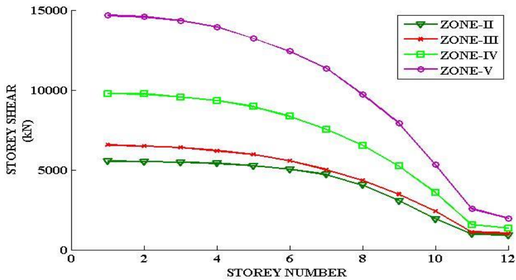
Fig: 7 Storey shear on shear wall due to seismic forces
