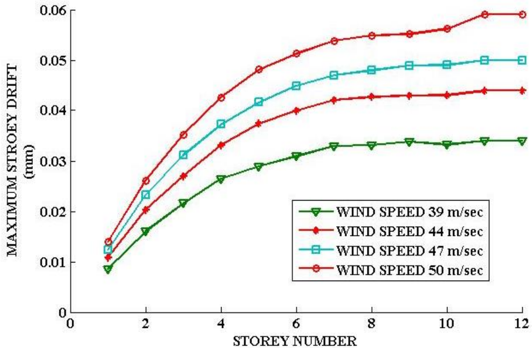
Fig: 11 Maximum storey drift on shear wall due to wind forces
