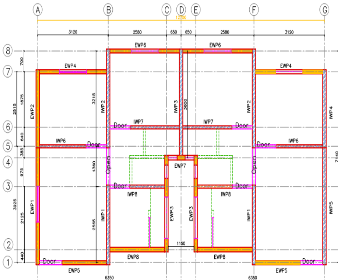
Fig.1 A typical two flats floor plan of structure
